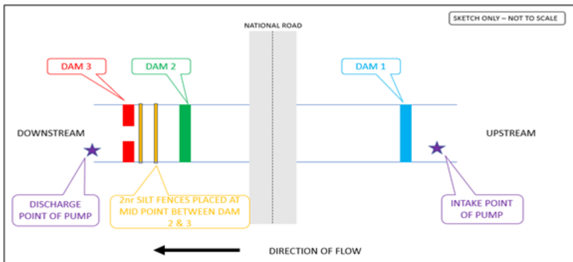
Figure 3-2 - Schematic of three dam dewatering system proposed at Carrowrevagh Bridge.
